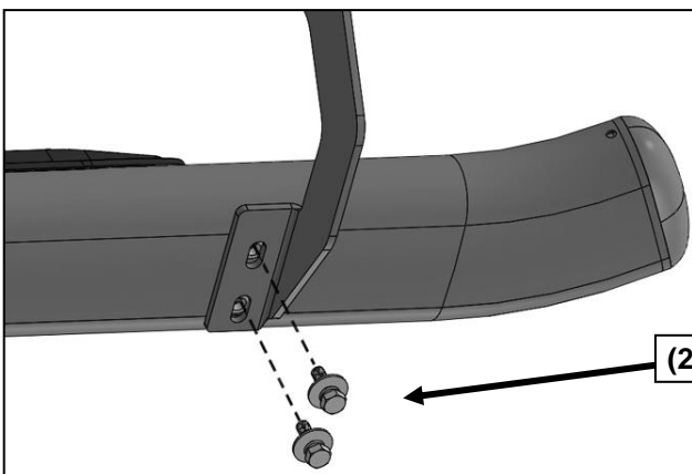
(Fig 8) Sidebar attached to Mounting Bracket
